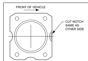
Figure 4. Flange Modifications
