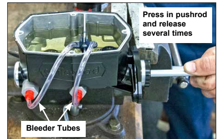
Typical Bleeder Tube Setup and Use
