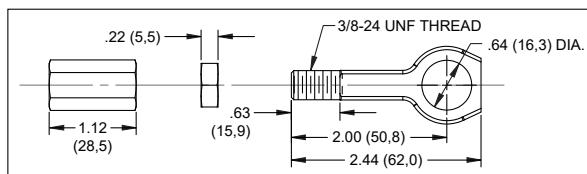
MOPAR PUSH ROD - EYELET DETAIL
