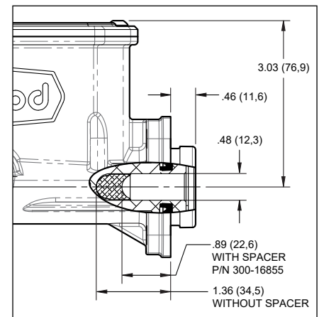
Master Cylinder Piston Detail
