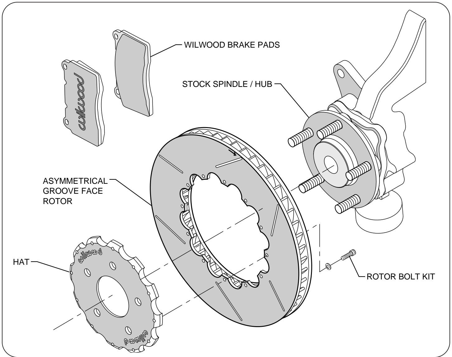
Typical Installation Diagram, Major Components Identified
