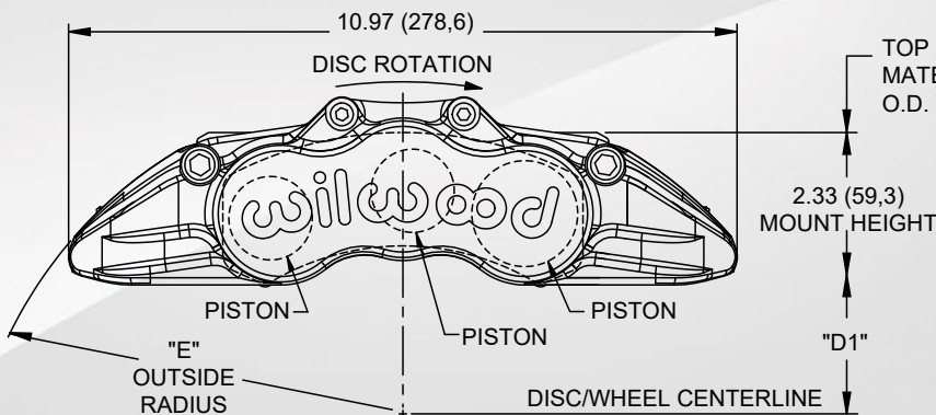
GN6R Caliper, Dimensional Characteristics
