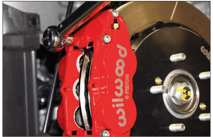
Sequence 23: Secure the caliper with washer and locknut, temporarily tighten. View the rotor through the top opening of the caliper. The rotor should be centered in the caliper. If not, adjust by adding or subtracting shims between the bracket and the mounting ears. Once the caliper alignment is correct, remove the bracket bolts one at a time and apply red Loctite ® 271 to the threads and torque to 65 ft-lb.
