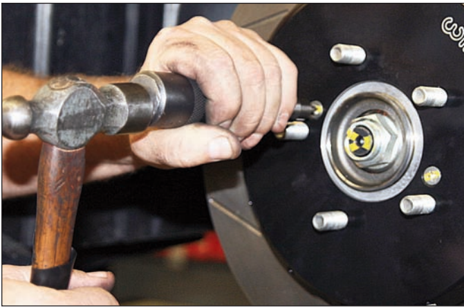
Sequence 19: Reinstall the hat locator screws using an impact screw driver to keep the hat/rotor in place while continuing with the rest of the installation.
