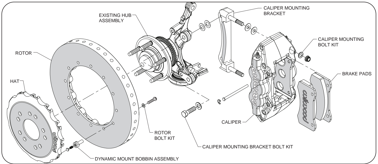
Front WCCB Kit, Typical Installation
