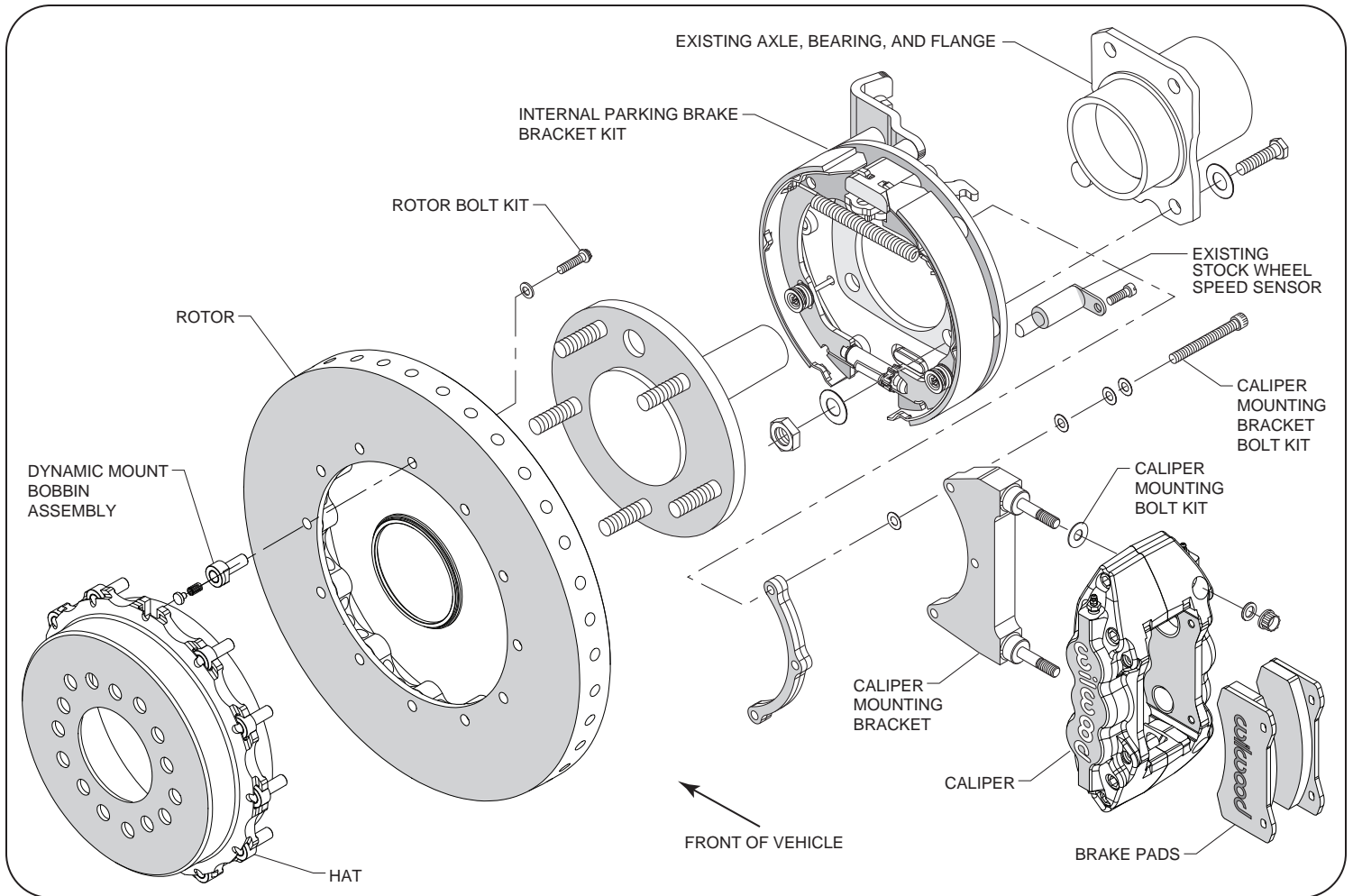
Rear WCCB Kit, Typical Installation
