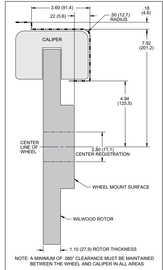
Figure 4. Wheel Clearance Diagram
