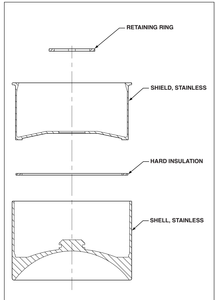
CONSTRUCTION DIAGRAM
