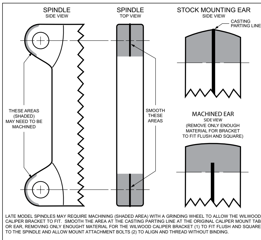
Figure 3. Machining Diagram
