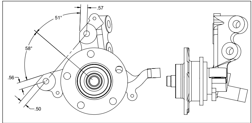
Figure 3. Spindle Modifications
