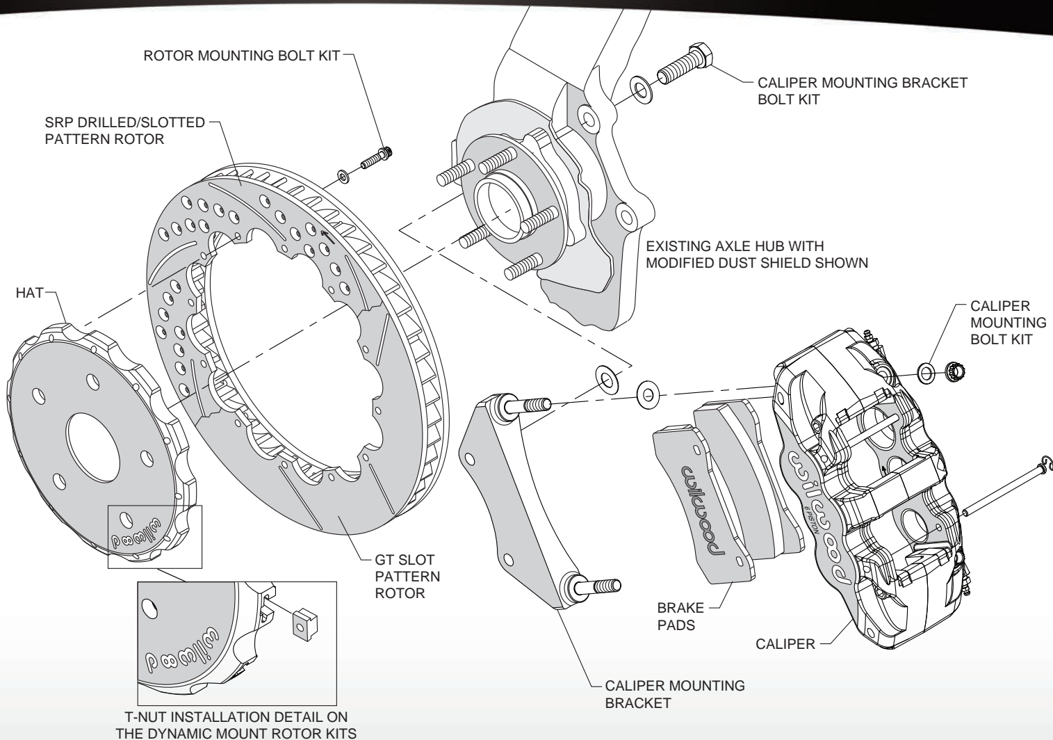
Figure 1. Typical Installation Diagram
