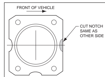
Figure 4. Flange Modifications
