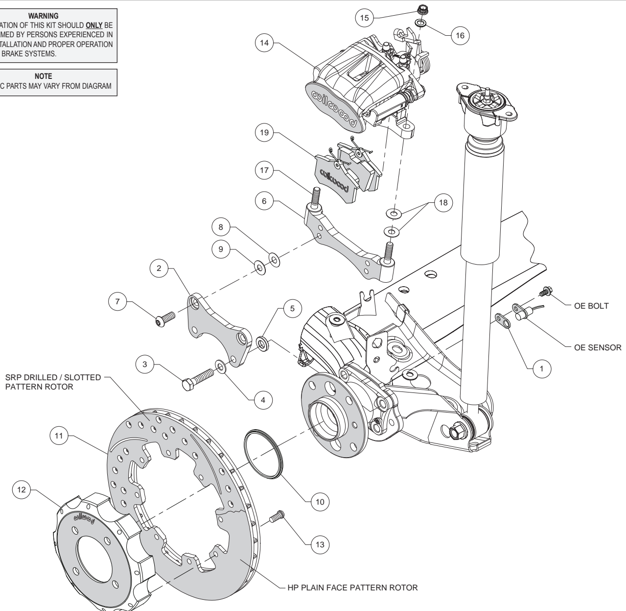
Figure 1. Typical Installation Configuration
