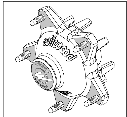
Starlite "55" Front Snap-Cap Hub
