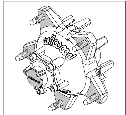
Starlite "55" Rear Hub with 5 Bolt Drive Flange
