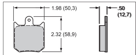
DLS Caliper, Type 7012 Pad Dimensions
