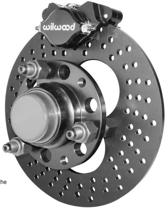
Dynalite Single Caliper with Drilled Solid Rotor
