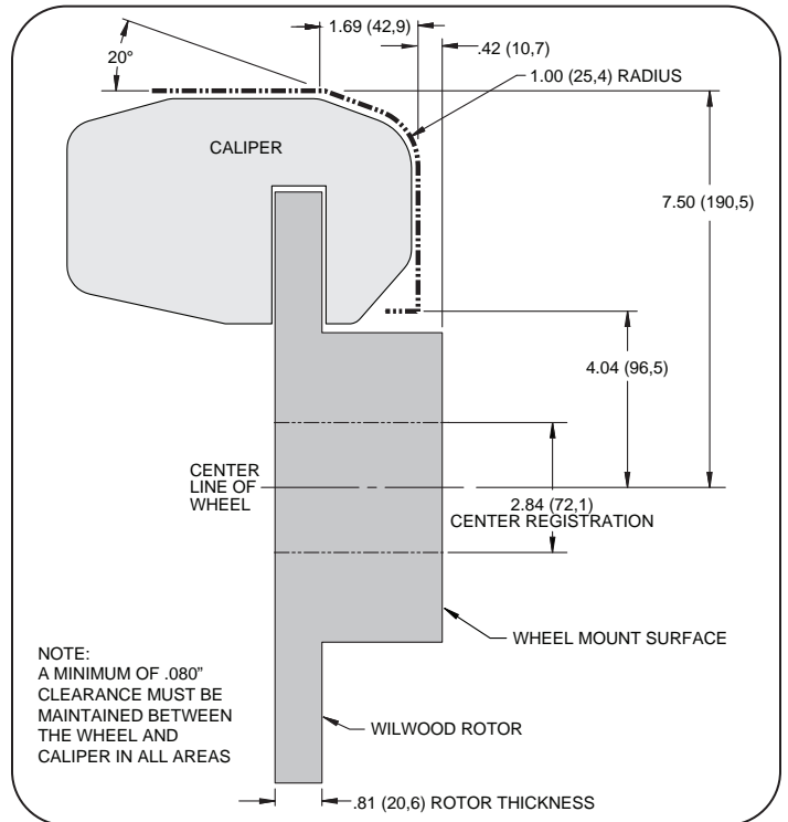
Wheel Clearance Diagram
