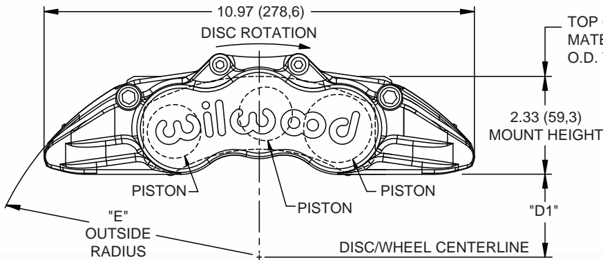
GN6R Caliper, Dimensional Characteristics
