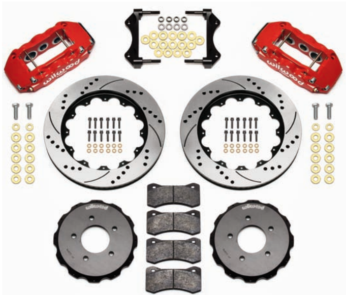
Front Big Brake Kit Components with Optional Red Calipers and Drilled Rotors
