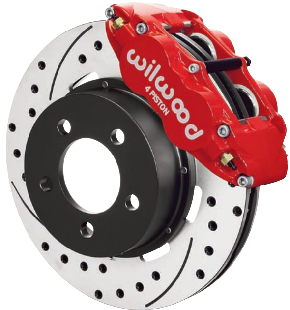
Front Jeep Brake Kit Assembly Download High Resolution Photo, Click Here
