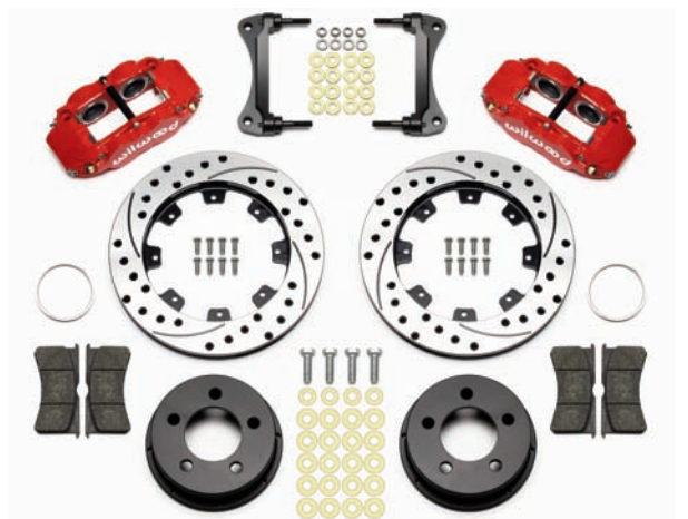
Rear Jeep Complete Brake Kit Download High Resolution Photo, Click Here
