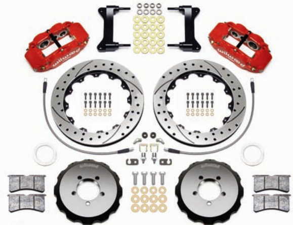
Subaru Complete Brake Kit, 13.06" Kit Shown Download High Resolution Photo, Click Here
