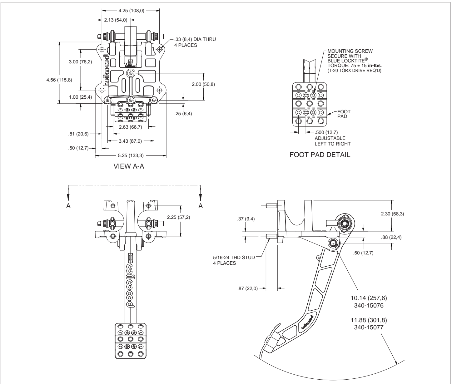
Figure 1. Reverse Mount Single Pedal Assembly, Physical Dimensions (P/N 340-15076 and 340-15077)
