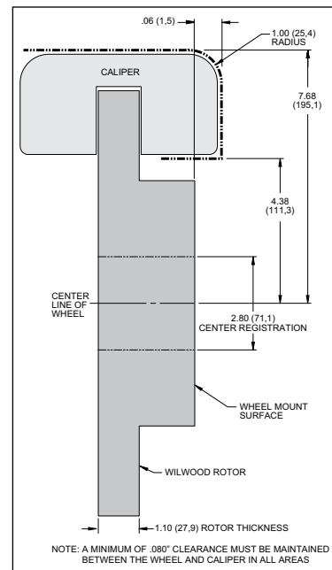
Figure 3B, P/N 140-16131. Wheel Clearance Diagram
