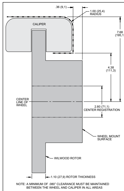
Figure 3A, P/N 140-15844. Wheel Clearance Diagram
