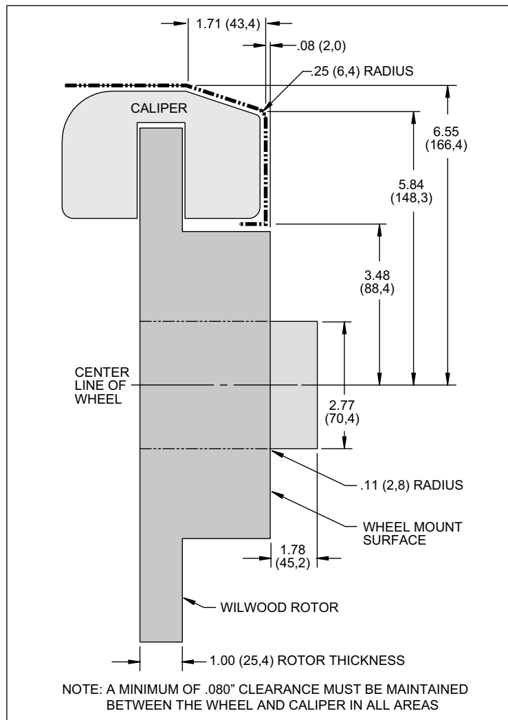
Figure 2. Wheel Clearance Diagram
