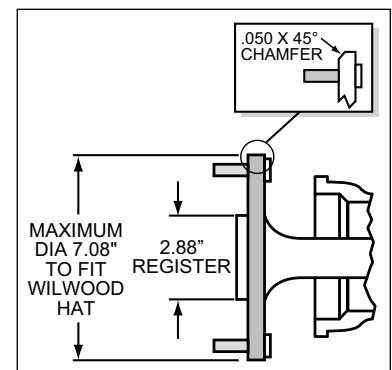
Figure 2. Axle Flange Maximum Dimension
