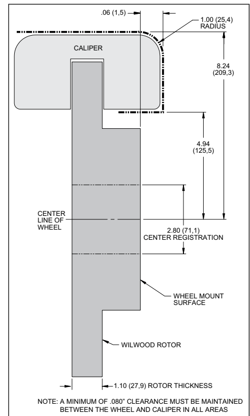
Figure 3. Wheel Clearance Diagram
