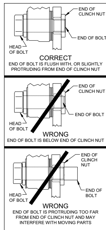
Figure 6. Clinch Nut Engagement Diagram
