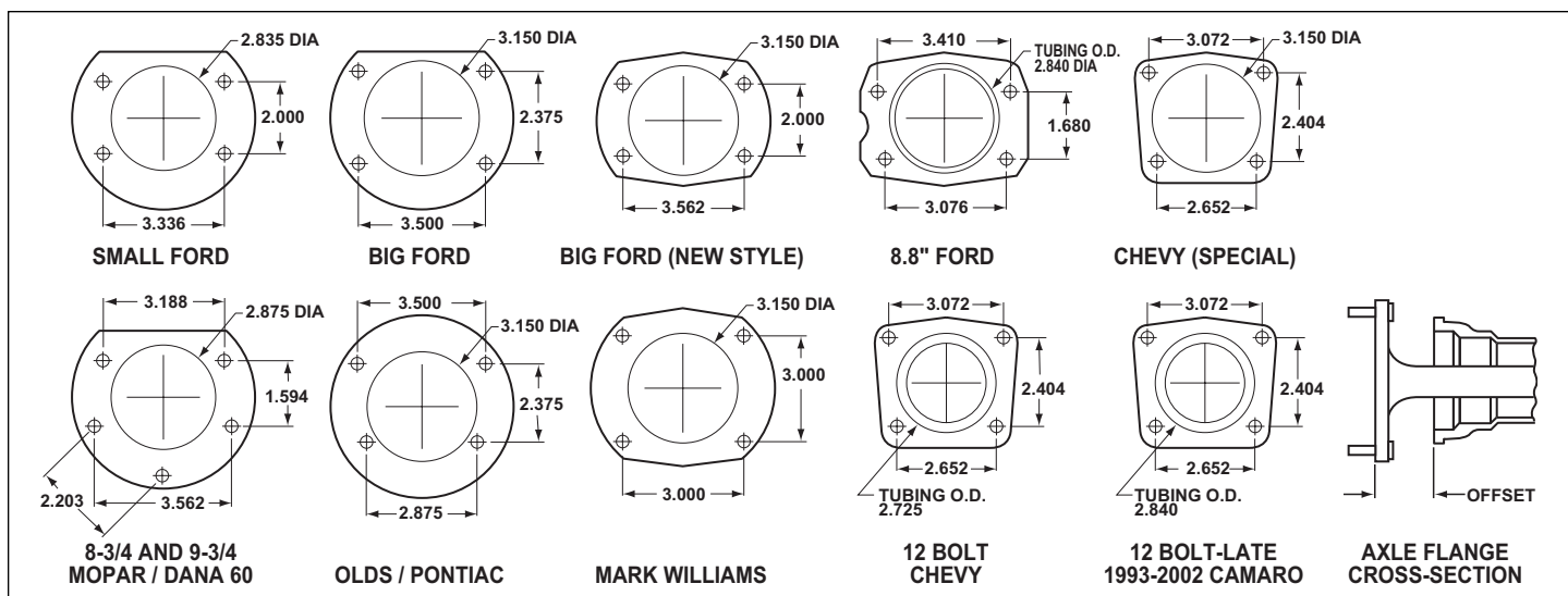
Figure 6. Rear Housing Flange Chart and Axle Flange / Offset Cross-Section
