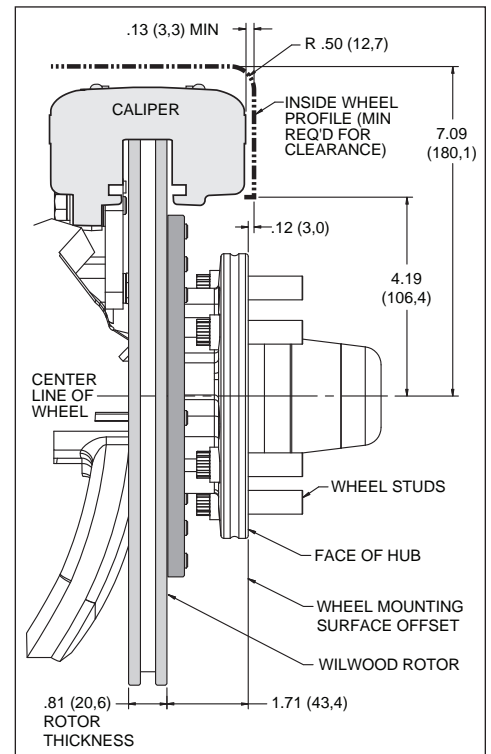
Figure 3. Wheel Clearance Diagram
