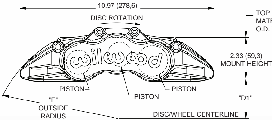
GN6R Caliper, Dimensional Characteristics
