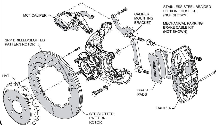
AERO4/MC4 Rear, Spec37 GTB Slotted Rotor
