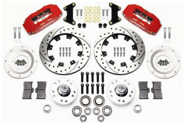
Complete Brake Kit
