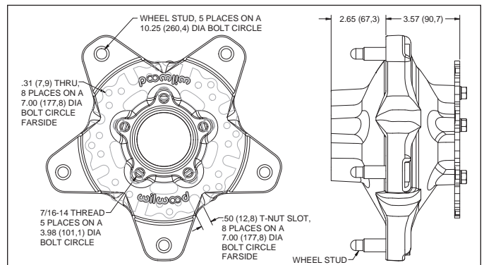
Starlite 55-XD Wide 5 Racing Hub, Dimensional Characteristics
